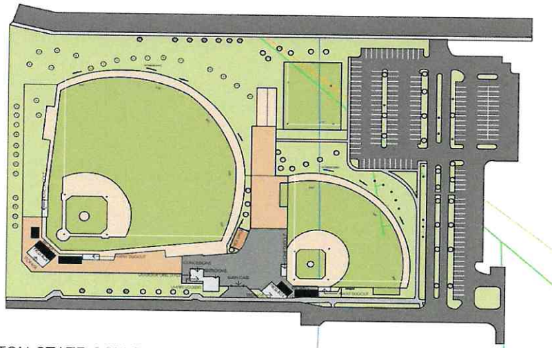
WILLISTON STATE COLLEGE TURF FIELDS SITE PLAN DESIGNED BY: [unreadable] ENGINEER: [unreadable]
