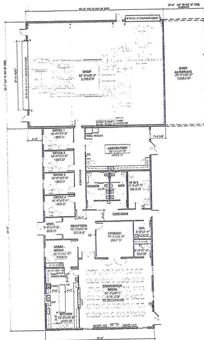
1 FLOOR PLAN SCALE: 1/8"=1'-0"
