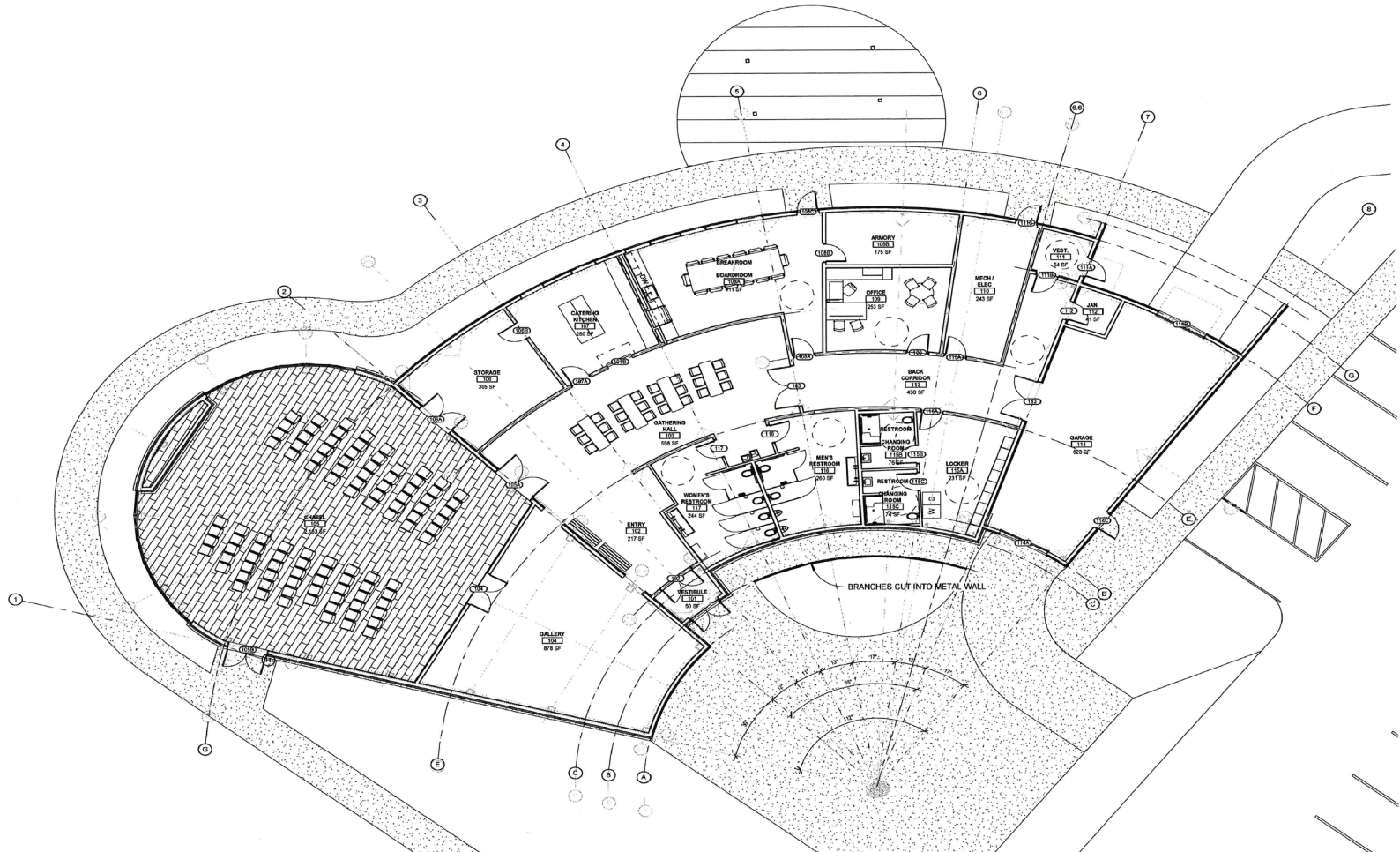
1 | A101 First Floor Plan 18" x 24"
