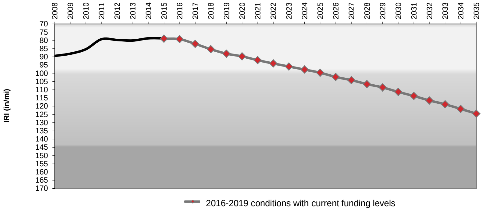
Average Network Condition - IRI
