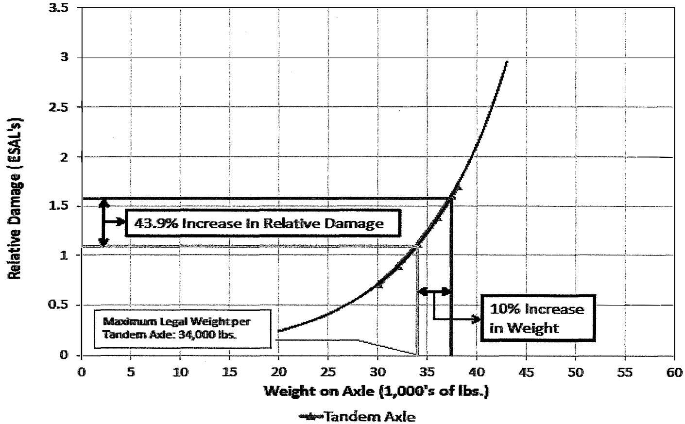
Tandem Axle: Relative Damage vs. Axle Weight
