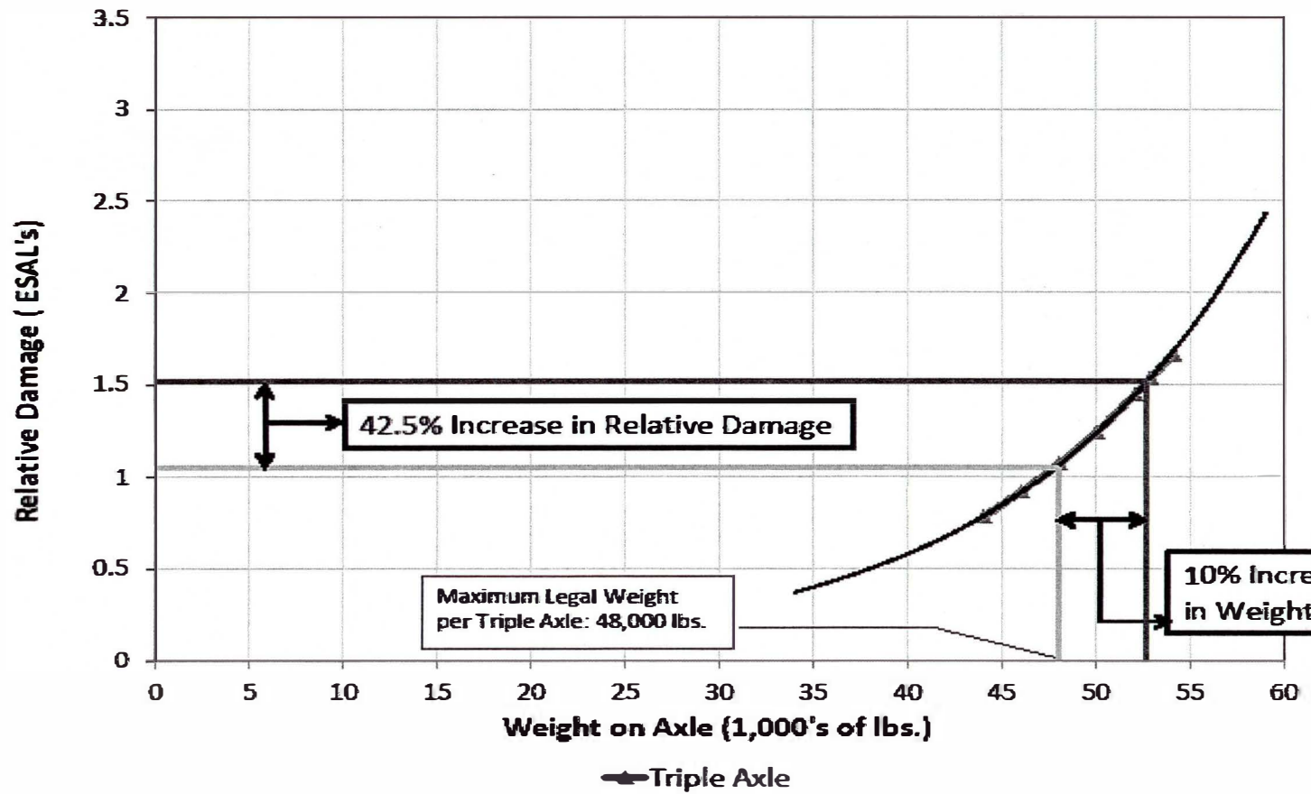
Triple Axle: Relative Damage vs. Axle Weight
