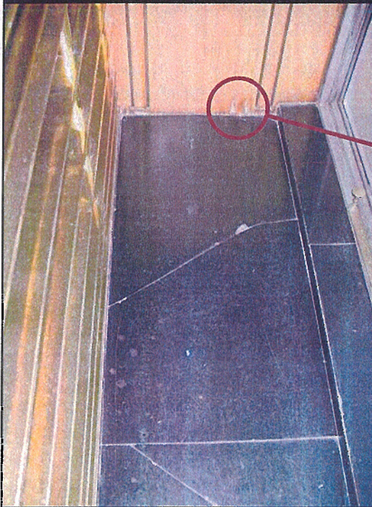
Window Sill @ West End of Legislative Wing showing Cracked Marble and Delaminated Wood Sill/Jamb
