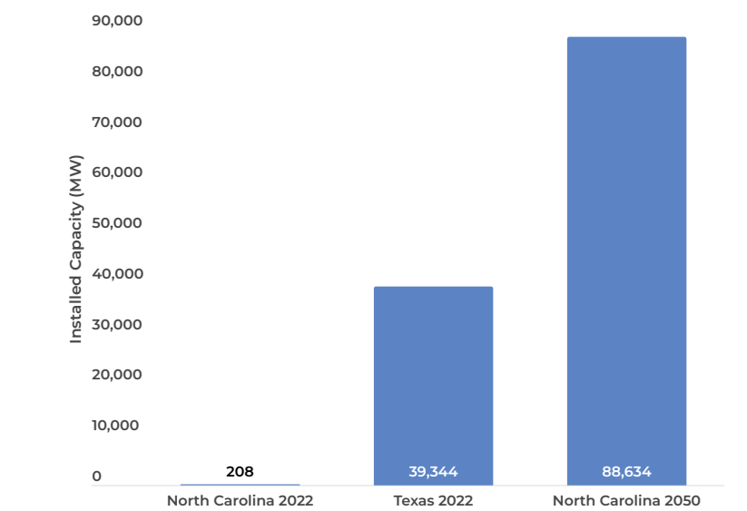
FIGURE 2.4 INSTALLED WIND CAPACITY IN NORTH CAROLINA UNDER THE RENEWABLE SCENARIO — COMPARISON WITH TEXAS
